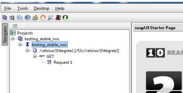
Figure 4. Project Tree.
