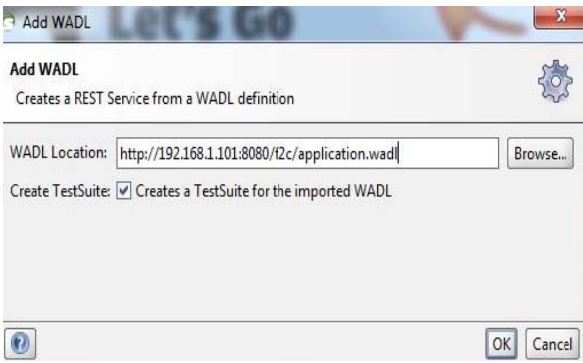
Figure 3. Linking WADL.
